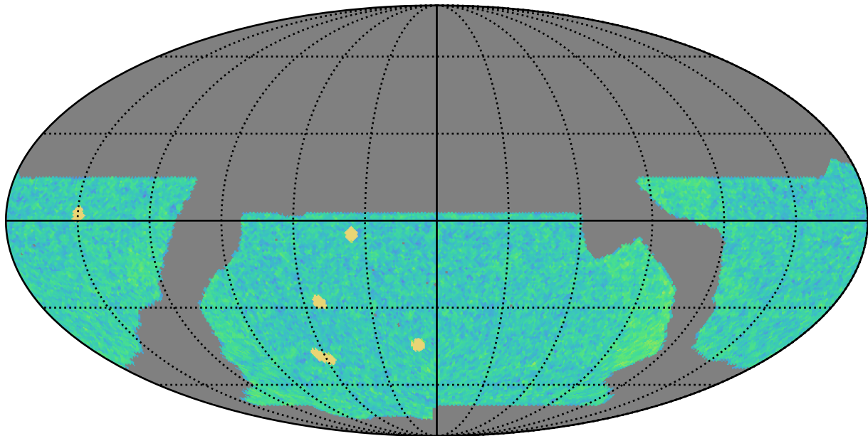
baseline_v2.1_10yrs WFD i band: NVisits
