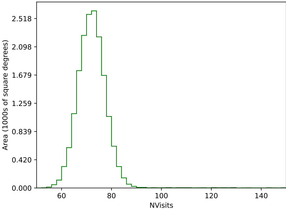
baseline_v2.1_10yrs WFD g band: NVisits
