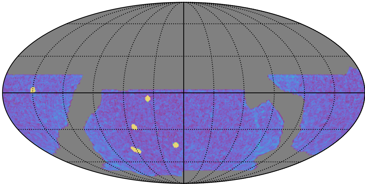
baseline_v2.1_10yrs WFD all bands: NVisits
