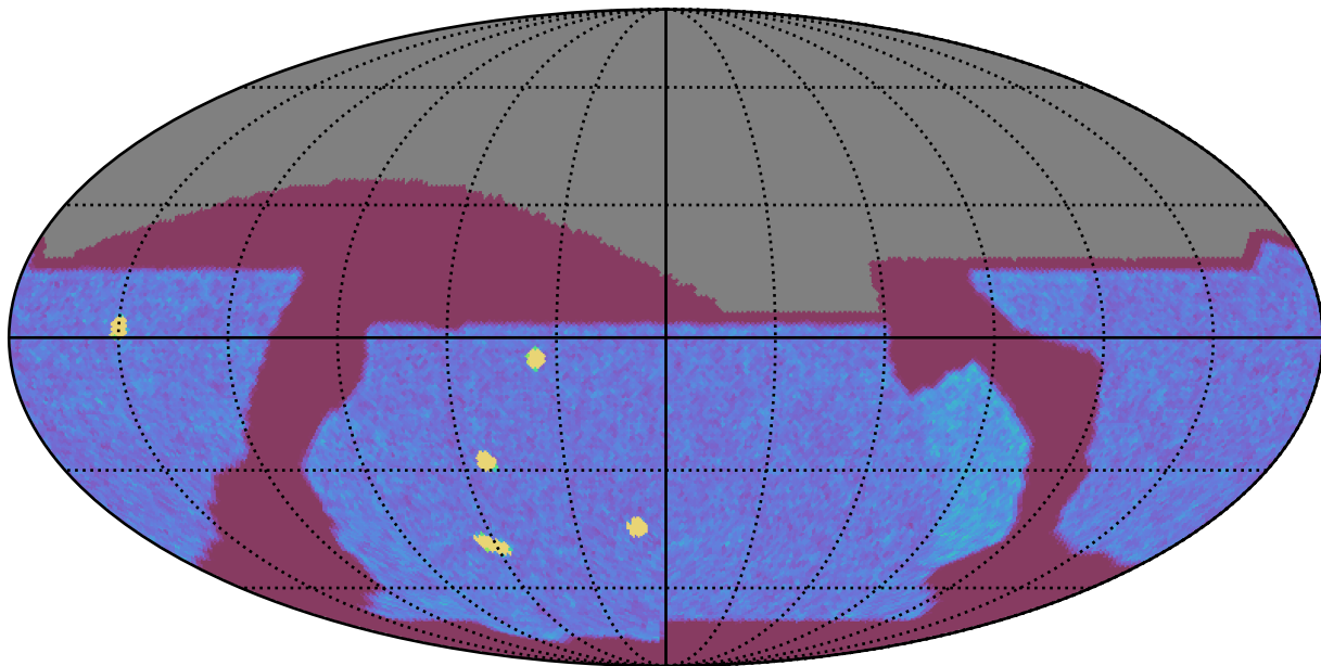
baseline_v2.1_10yrs All sky z band: NVisits
