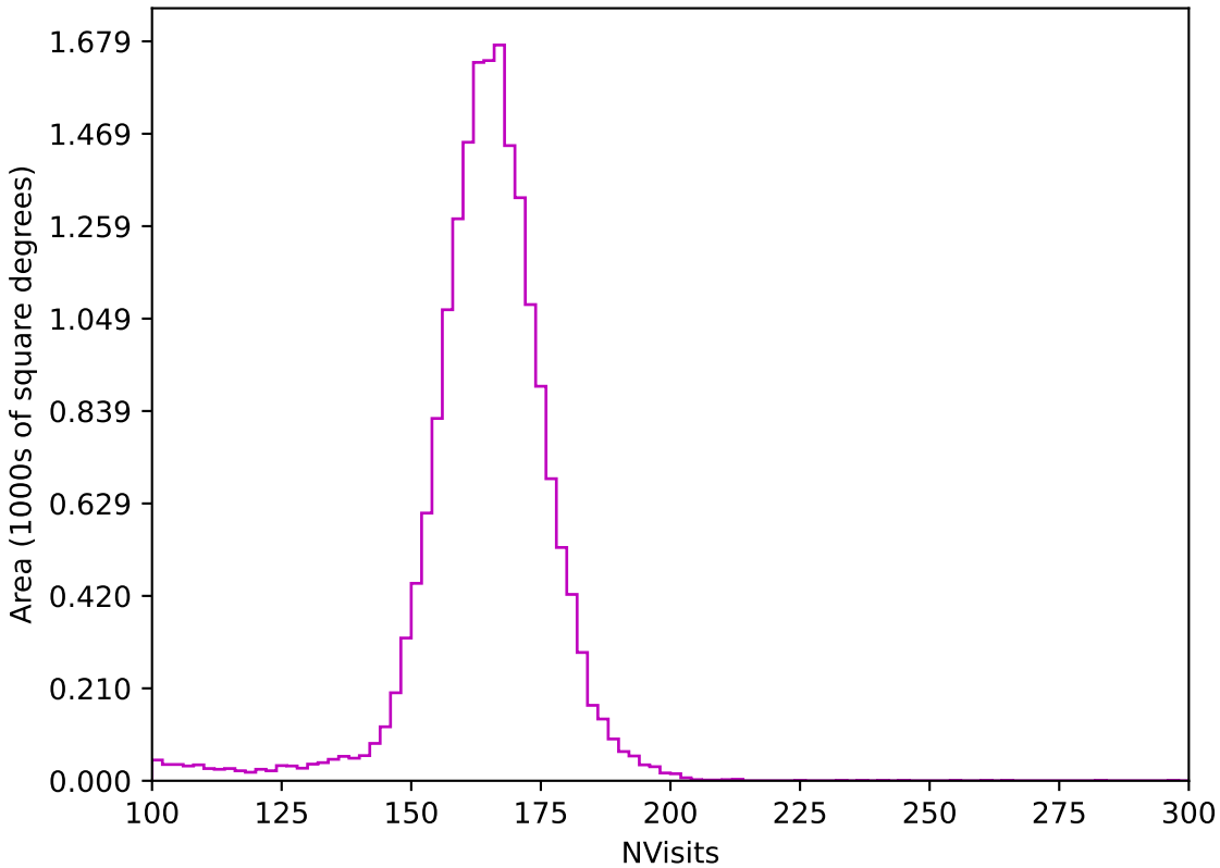
baseline_v2.1_10yrs All sky z band: NVisits
