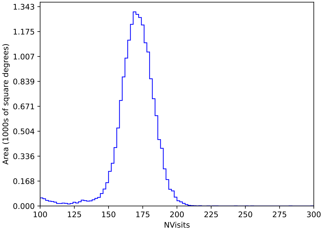
baseline_v2.1_10yrs All sky y band: NVisits
