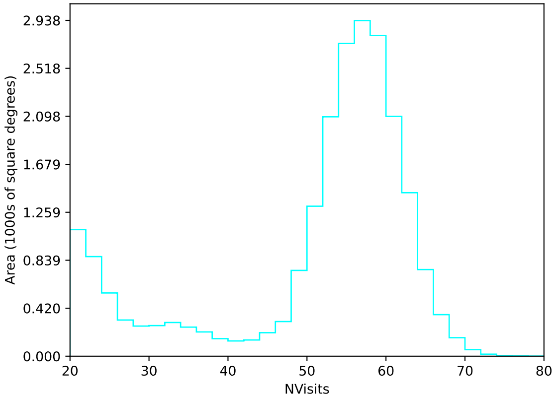
baseline_v2.1_10yrs All sky u band: NVisits
