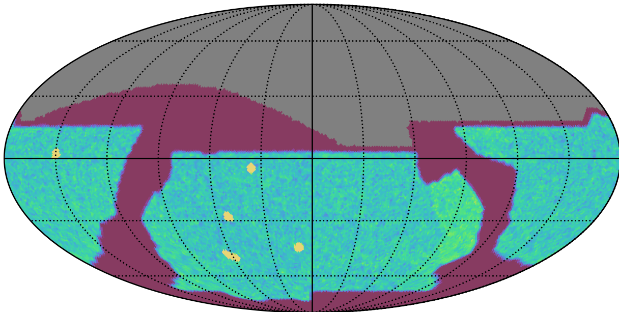
baseline_v2.1_10yrs All sky r band: NVisits
