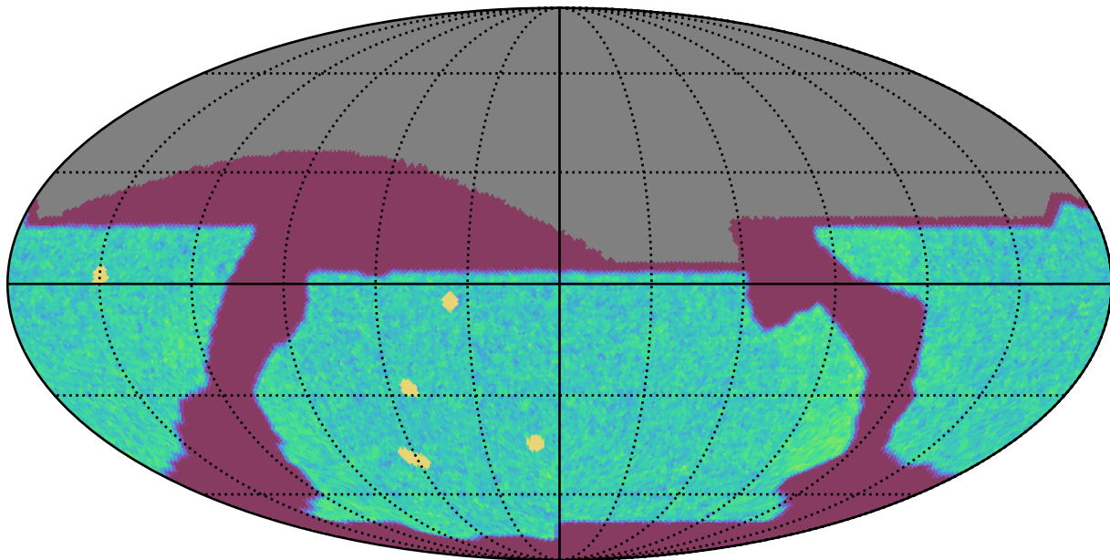
baseline_v2.1_10yrs All sky i band: NVisits
