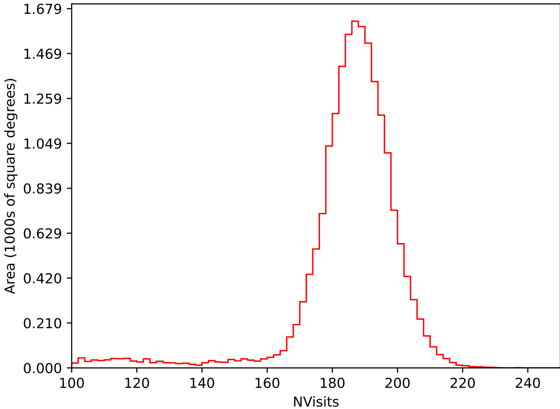
baseline_v2.1_10yrs All sky i band: NVisits
