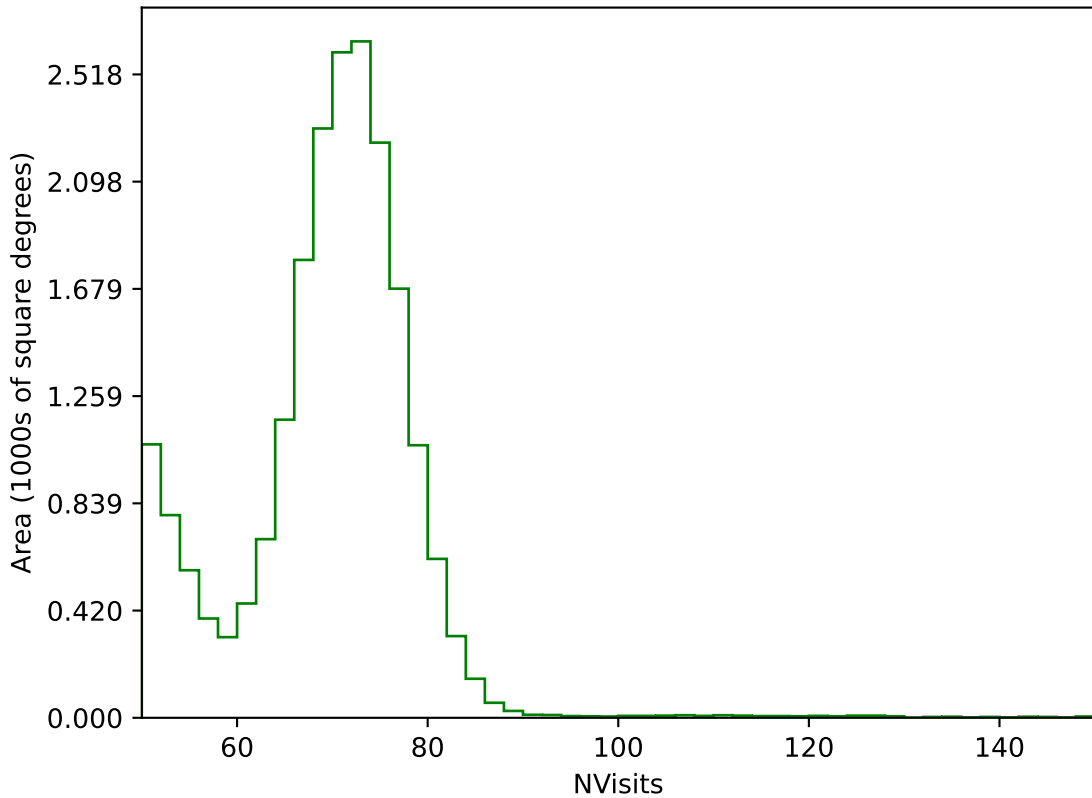
baseline_v2.1_10yrs All sky g band: NVisits
