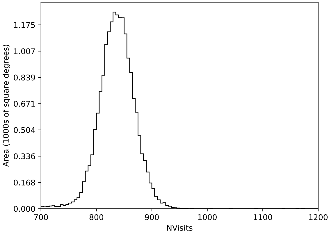
baseline_v2.1_10yrs All sky all bands: NVisits
