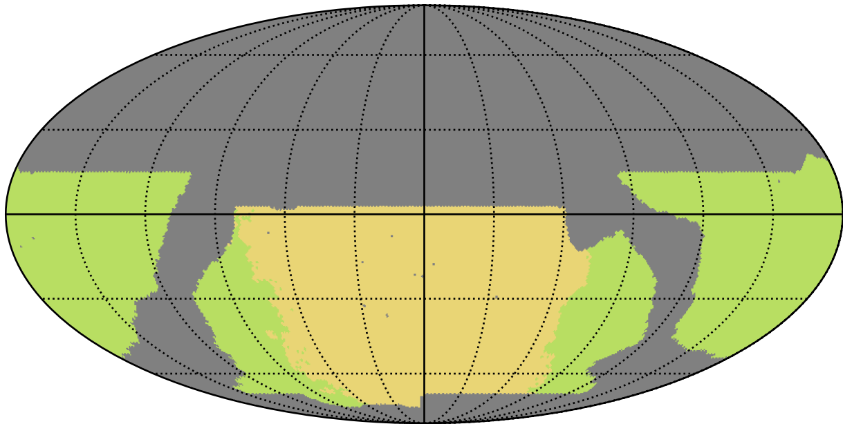
baseline_v2.1_10yrs WFD all bands: NSeasons
