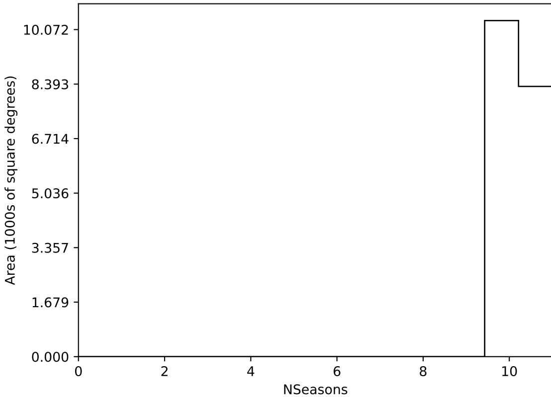
baseline_v2.1_10yrs WFD all bands: NSeasons
