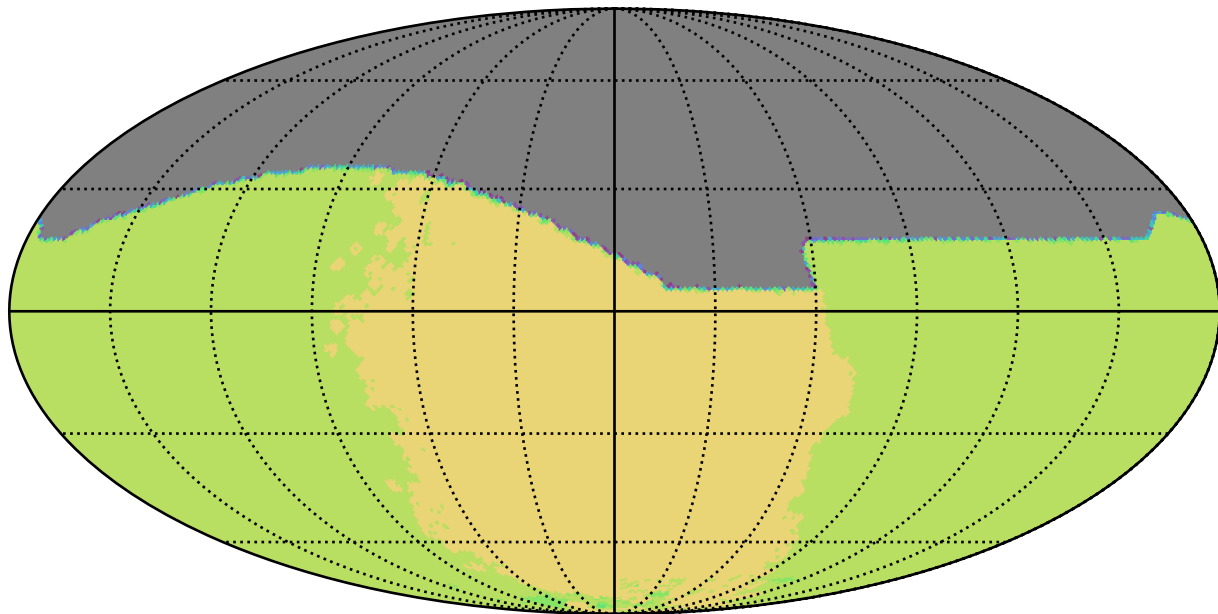
baseline_v2.1_10yrs All sky all bands: NSeasons
