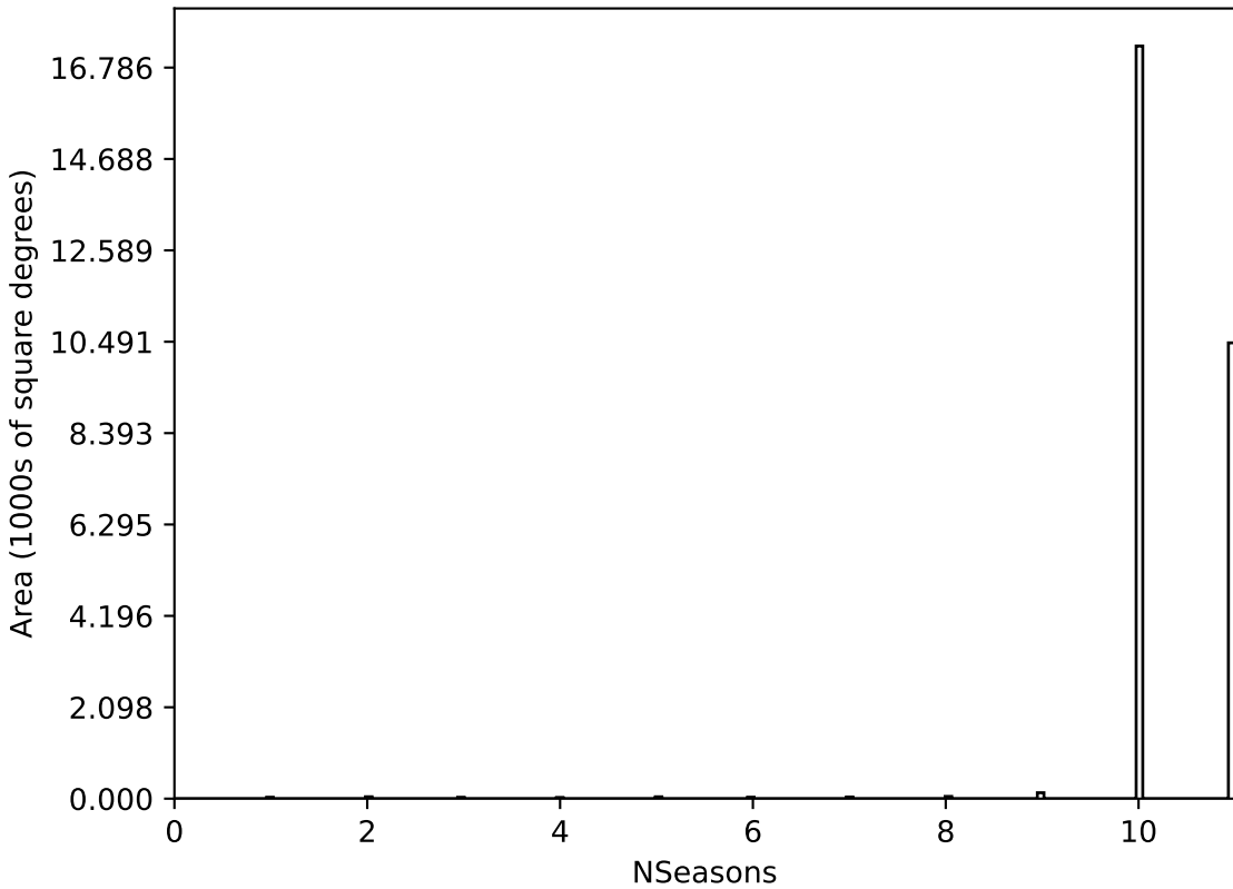
baseline_v2.1_10yrs All sky all bands: NSeasons
