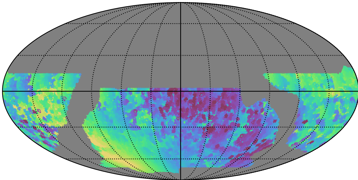
baseline_v2.1_10yrs WFD z band: Min solarElong
