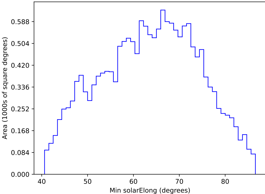
baseline_v2.1_10yrs WFD z band: Min solarElong
