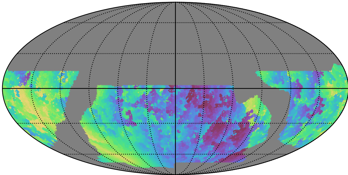
baseline_v2.1_10yrs WFD y band: Min solarElong
