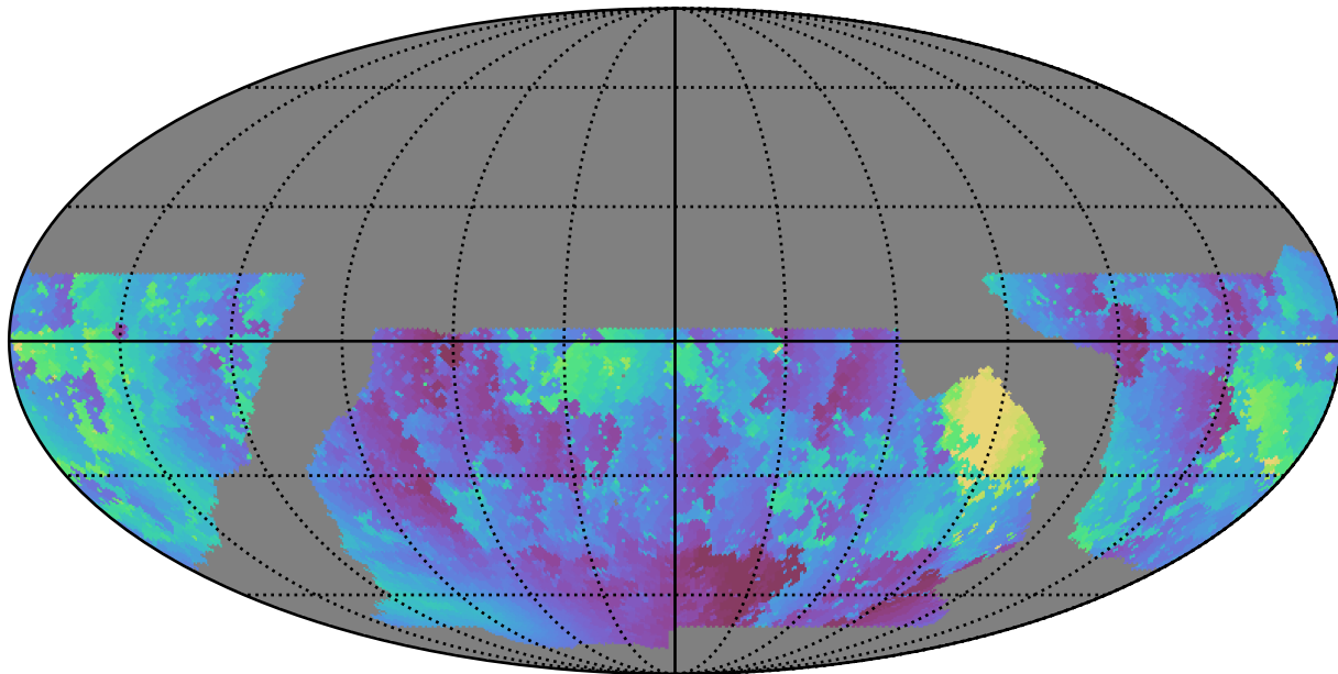
baseline_v2.1_10yrs WFD u band: Min solarElong
