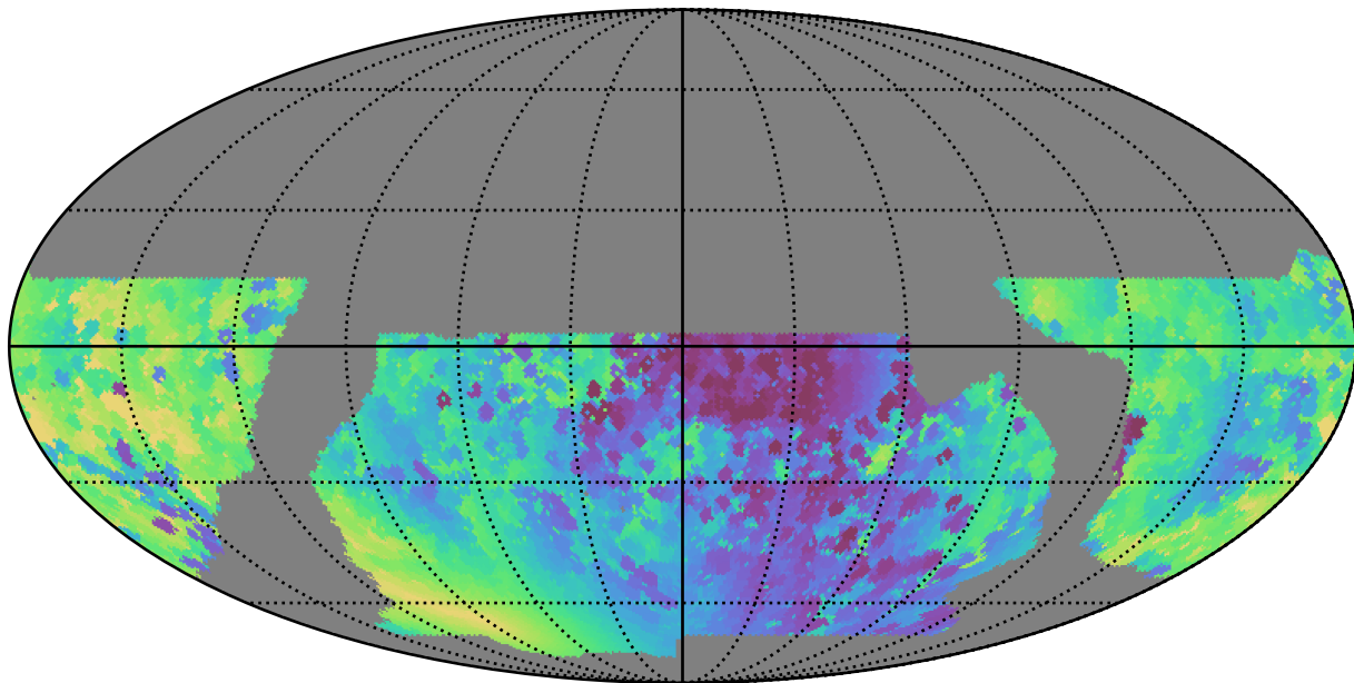
baseline_v2.1_10yrs WFD r band: Min solarElong
