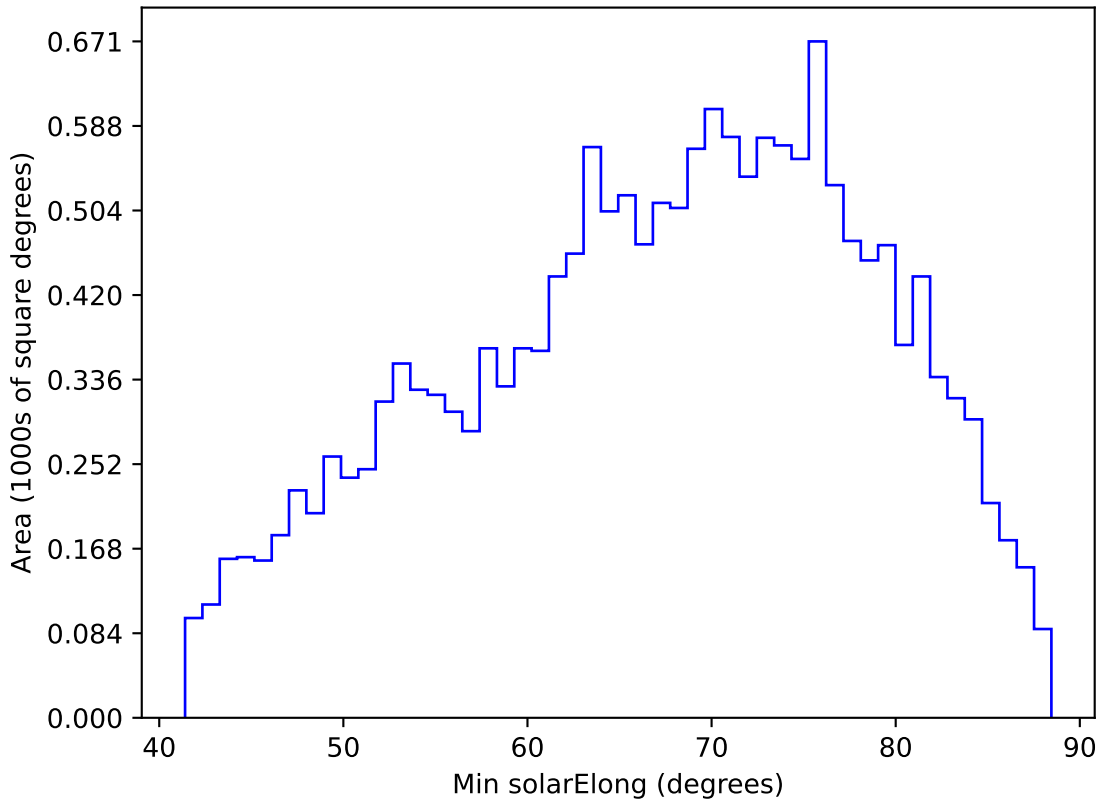
baseline_v2.1_10yrs WFD r band: Min solarElong
