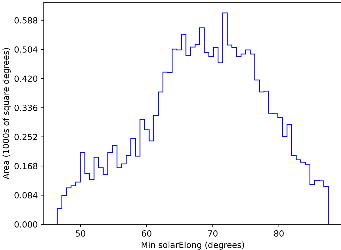
baseline_v2.1_10yrs WFD i band: Min solarElong
