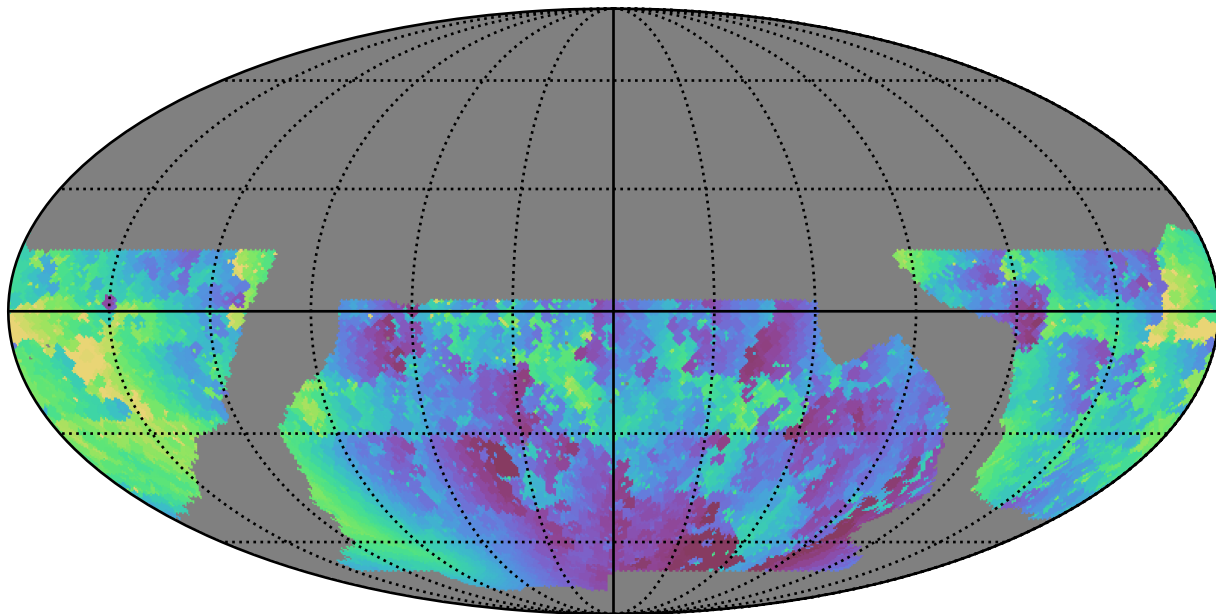
baseline_v2.1_10yrs WFD g band: Min solarElong
