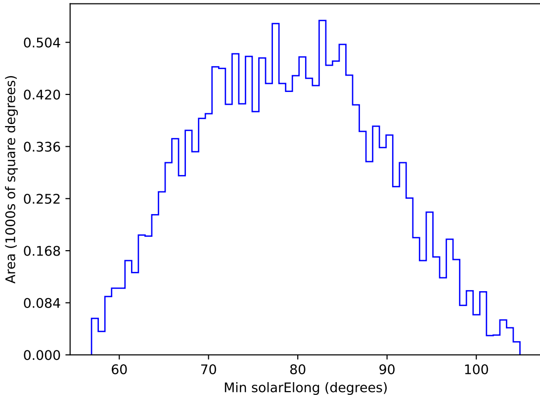
baseline_v2.1_10yrs WFD g band: Min solarElong
