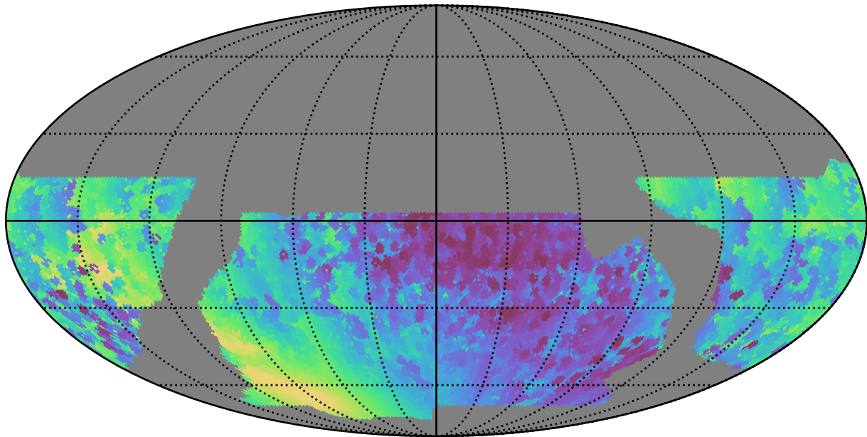
baseline_v2.1_10yrs WFD all bands: Min solarElong
