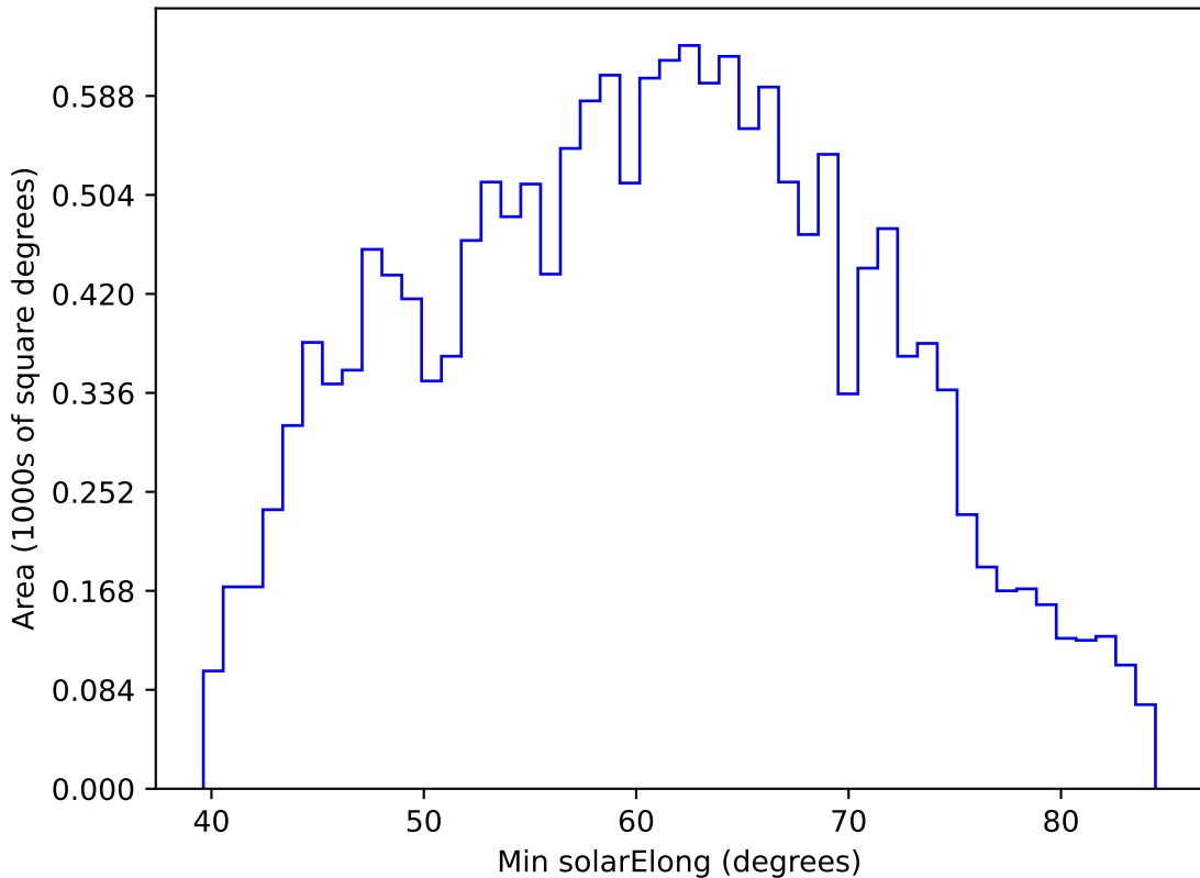
baseline_v2.1_10yrs WFD all bands: Min solarElong
