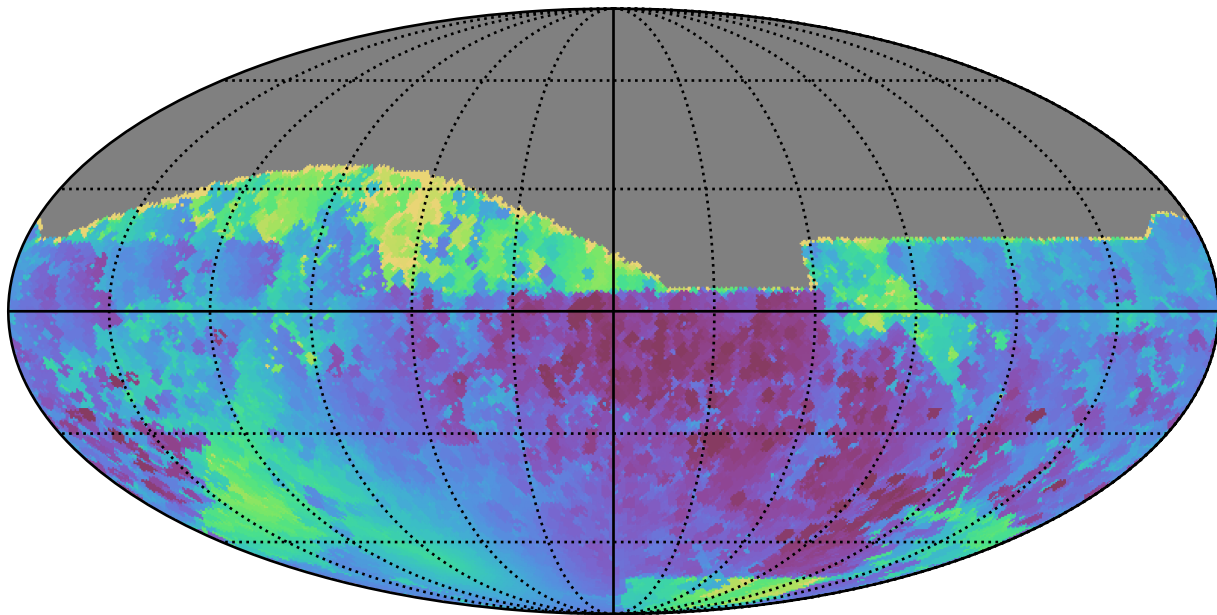
baseline_v2.1_10yrs All sky z band: Min solarElong
