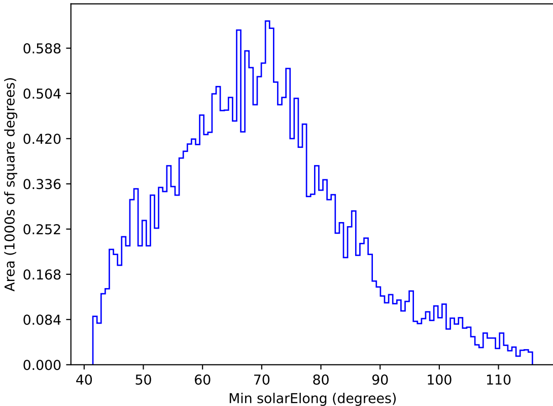
baseline_v2.1_10yrs All sky z band: Min solarElong
