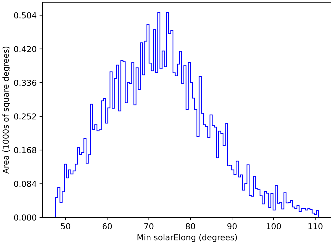
baseline_v2.1_10yrs All sky y band: Min solarElong
