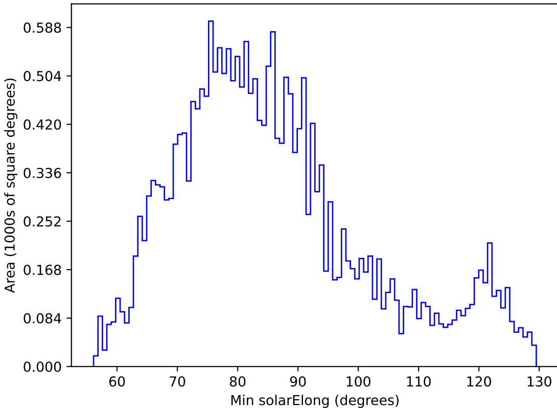
baseline_v2.1_10yrs All sky u band: Min solarElong
