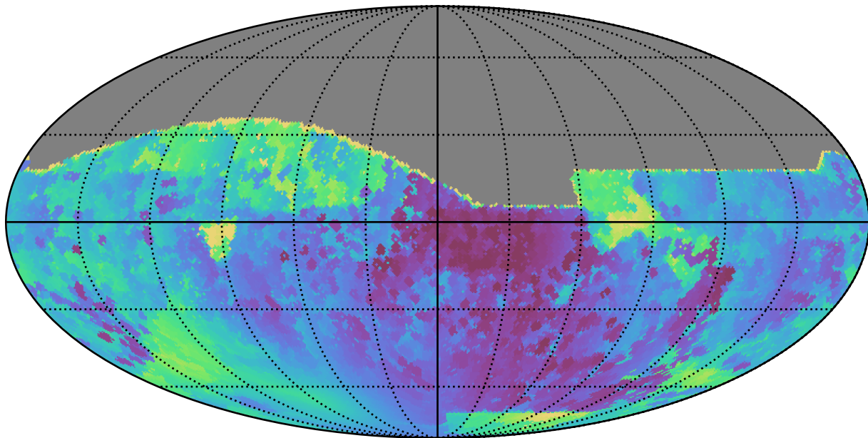
baseline_v2.1_10yrs All sky r band: Min solarElong
