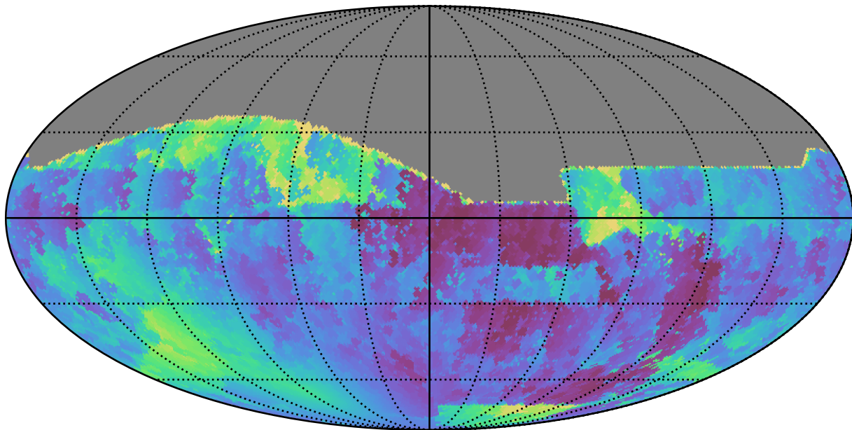
baseline_v2.1_10yrs All sky i band: Min solarElong
