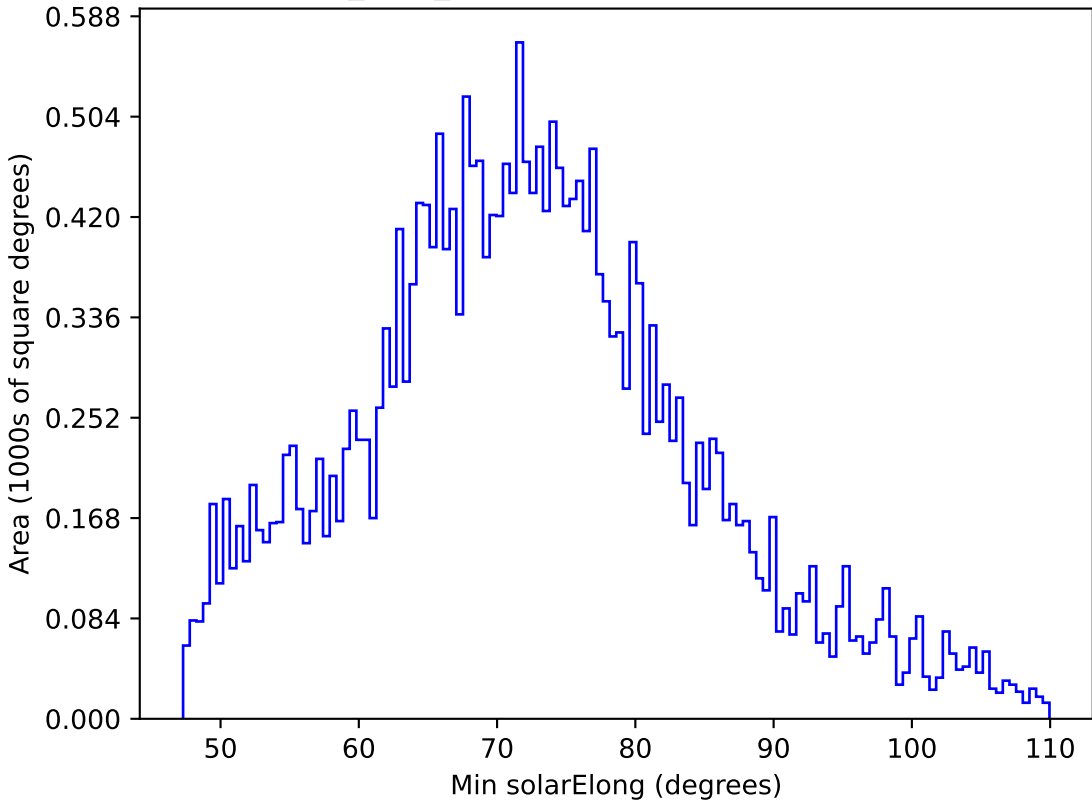
baseline_v2.1_10yrs All sky i band: Min solarElong
