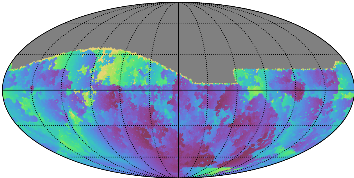
baseline_v2.1_10yrs All sky g band: Min solarElong
