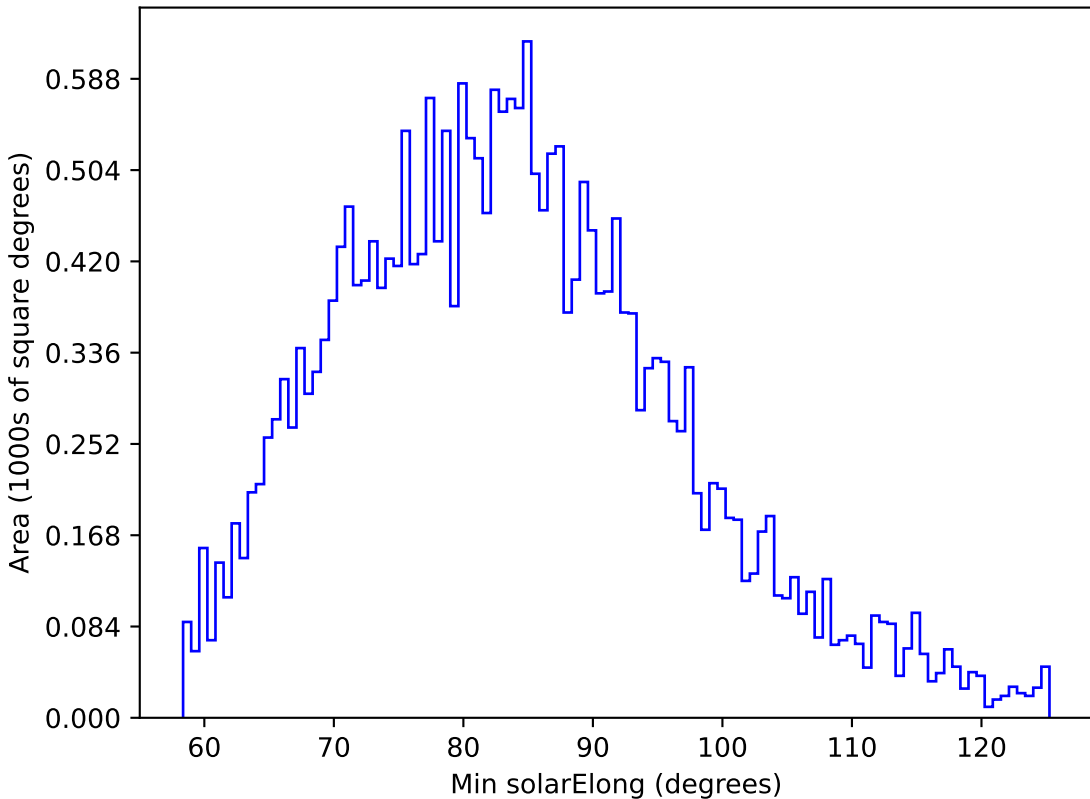
baseline_v2.1_10yrs All sky g band: Min solarElong
