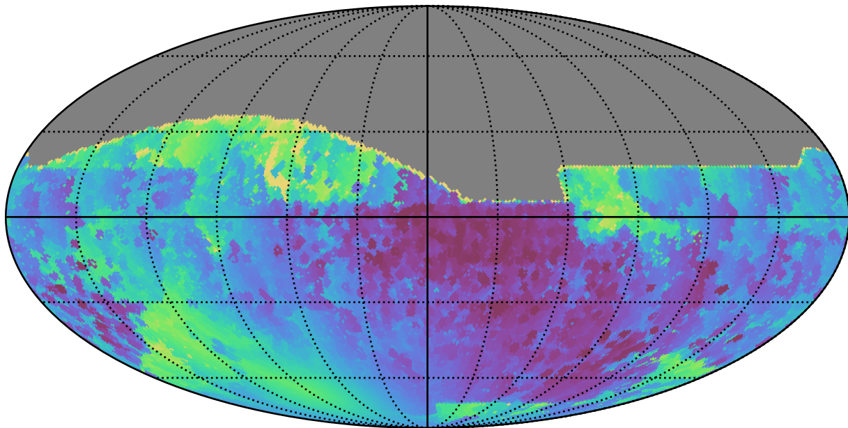
baseline_v2.1_10yrs All sky all bands: Min solarElong
