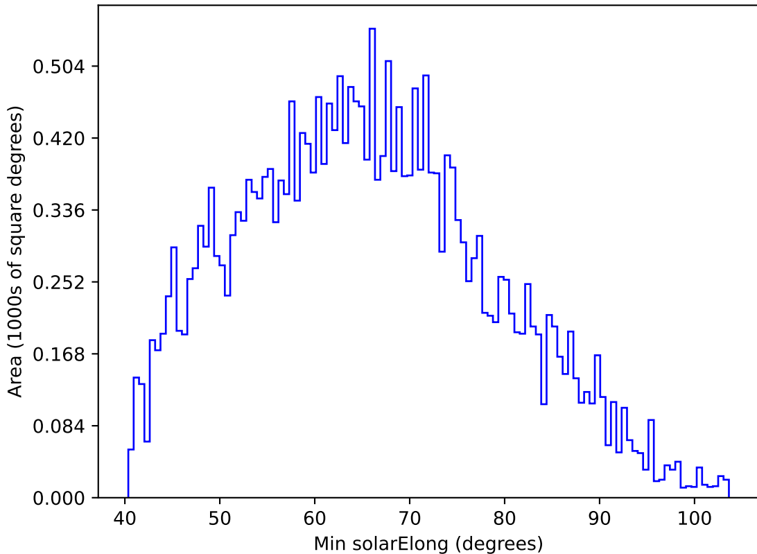
baseline_v2.1_10yrs All sky all bands: Min solarElong
