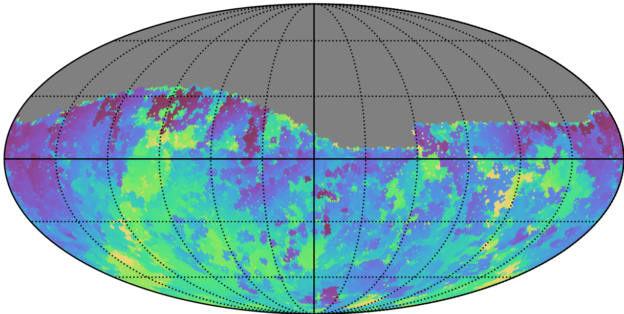
baseline_v2.1_10yrs Yr 1 z band: Min skyBrightness
