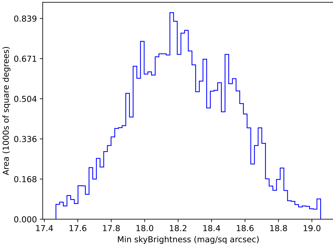
baseline_v2.1_10yrs Yr 1 z band: Min skyBrightness
