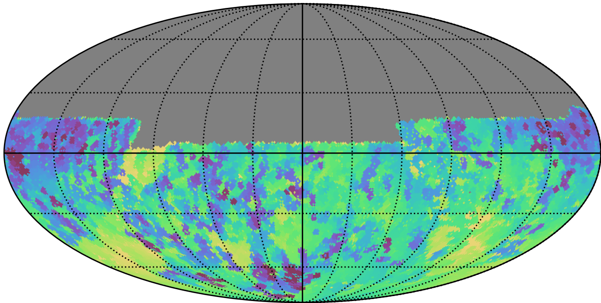
baseline_v2.1_10yrs Yr 1 y band: Min skyBrightness
