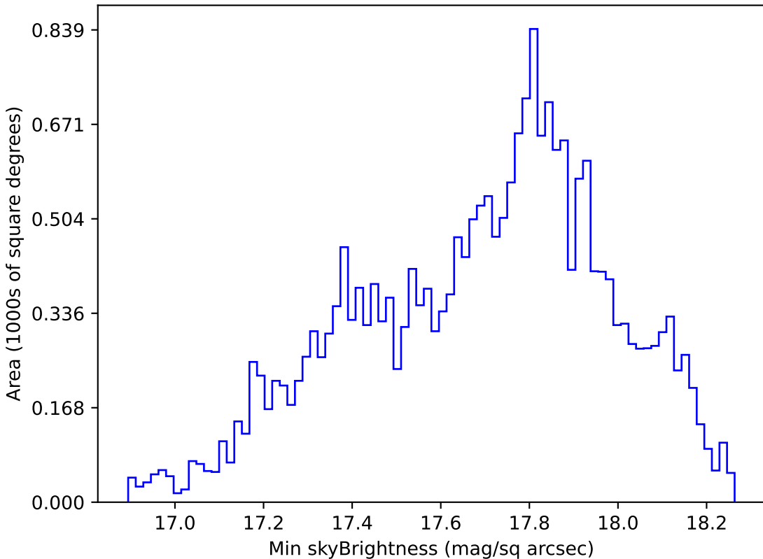
baseline_v2.1_10yrs Yr 1 y band: Min skyBrightness
