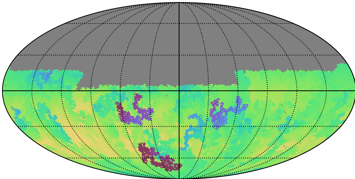
baseline_v2.1_10yrs Yr 1 u band: Min skyBrightness
