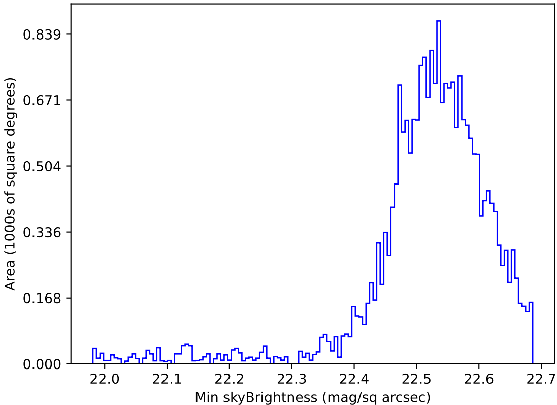
baseline_v2.1_10yrs Yr 1 u band: Min skyBrightness
