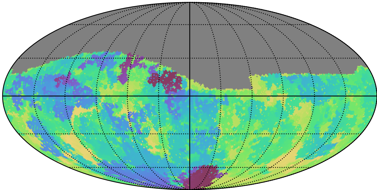
baseline_v2.1_10yrs Yr 1 r band: Min skyBrightness
