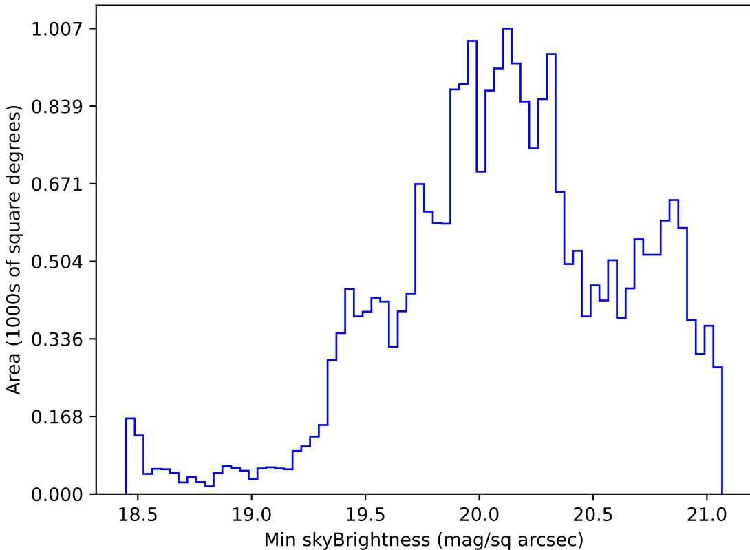
baseline_v2.1_10yrs Yr 1 r band: Min skyBrightness
