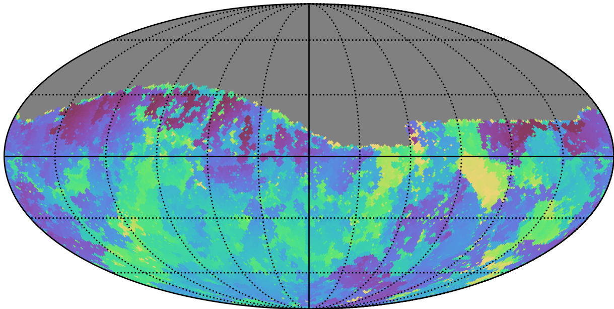
baseline_v2.1_10yrs Yr 1 i band: Min skyBrightness
