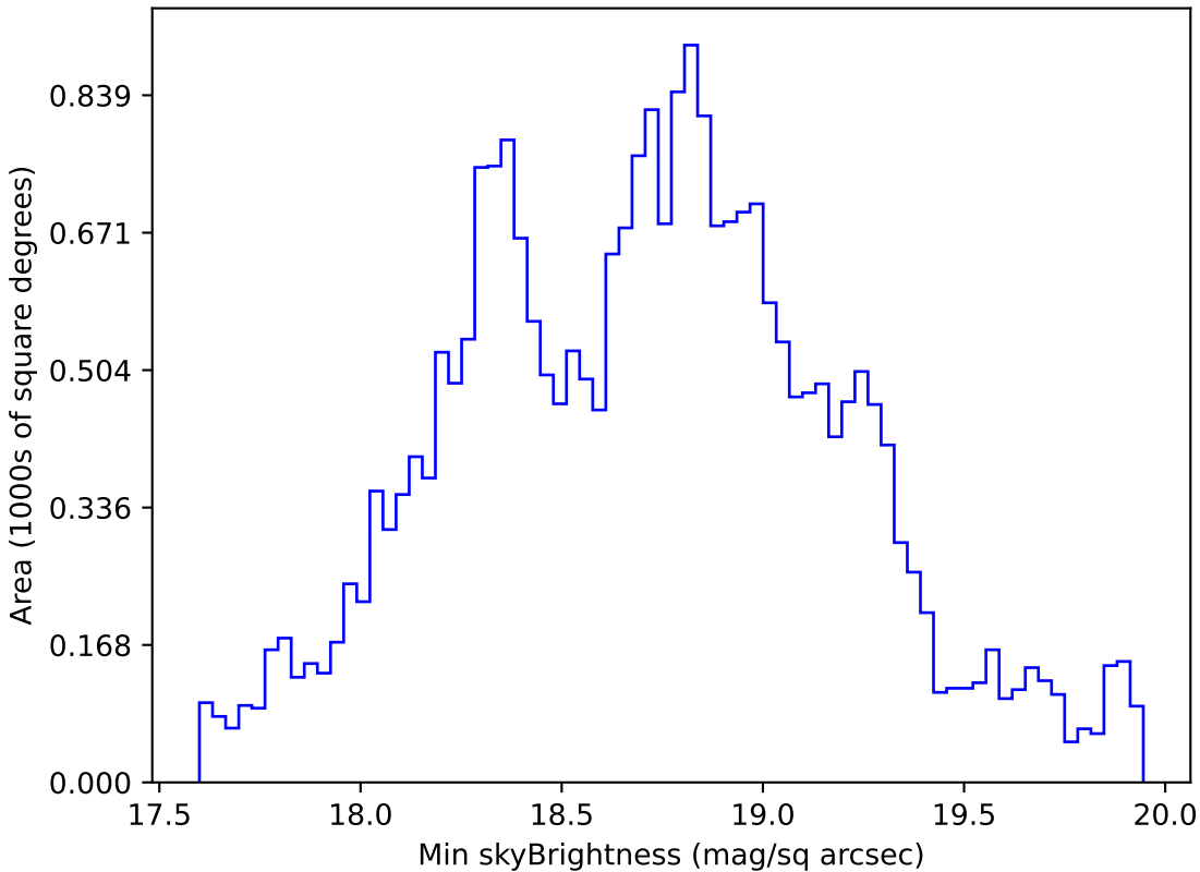
baseline_v2.1_10yrs Yr 1 i band: Min skyBrightness
