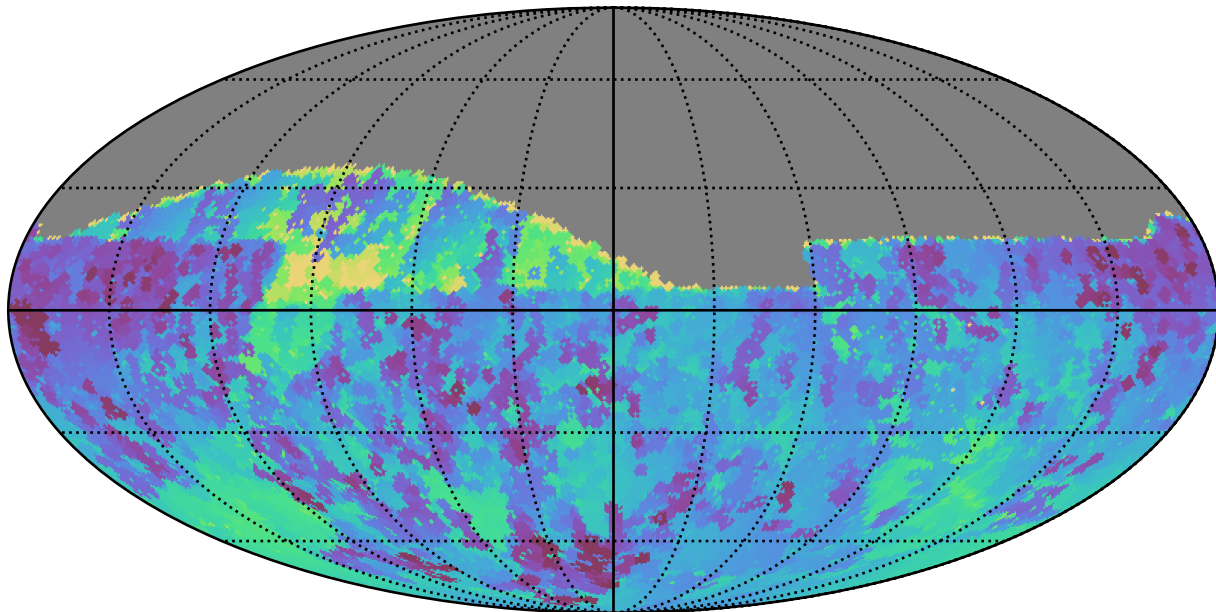
baseline_v2.1_10yrs Yr 1 all bands: Min skyBrightness
