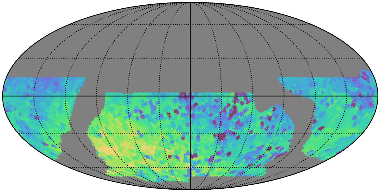
baseline_v2.1_10yrs WFD z band: Min skyBrightness
